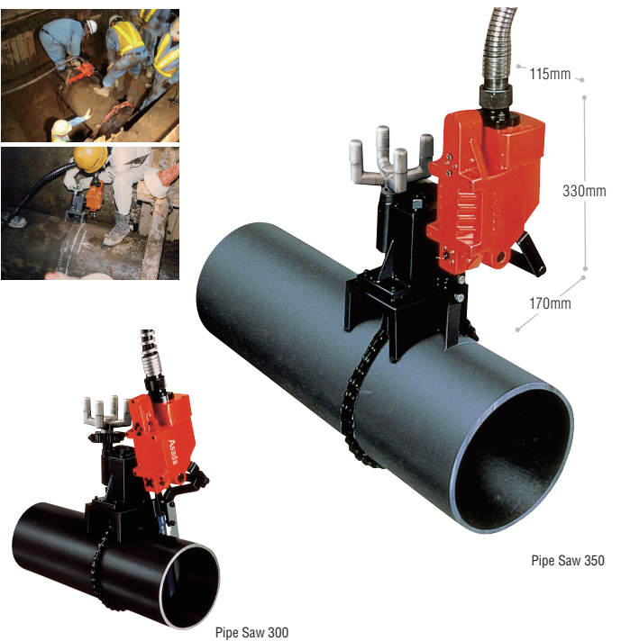
Pipe Saw 300
